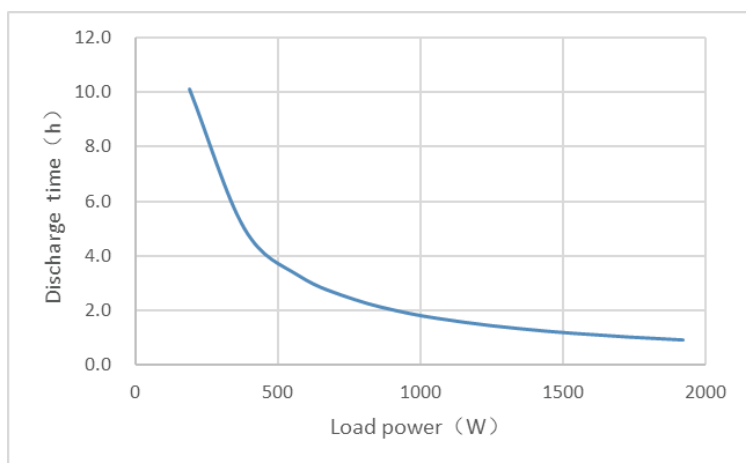
SDA10-4840 Discharge time at different load power
