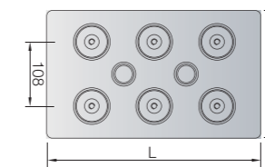
GFMJ-2000
