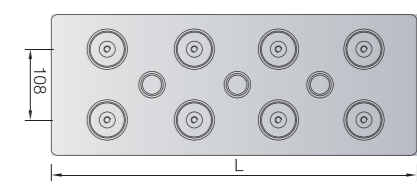
GFMJ-2500~GFMJ-3000
